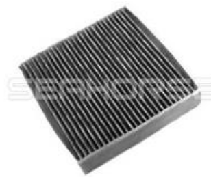
08975-K2000-100 Cabin Air Filter Seahorse No.: SC9044 Length : 185 mm Width : 178 mm Height : 30 mm
